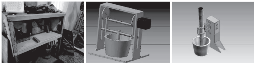
図3 「Original design [Left] First modified design [Center] Second modified design [Right]:Transition of design of a fufu pounder」(青木論文 p. 73 より転載)
